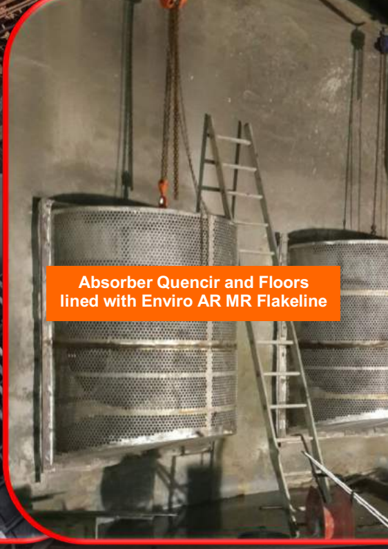
%98 Sulfuric Acid Absorber lined with Enviro AR MR Flakeline
